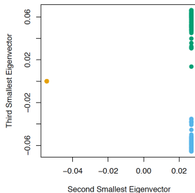
Spectral Clustering
